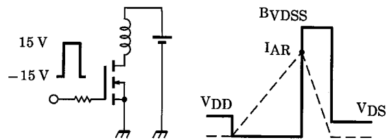
TEST CIRCUIT
